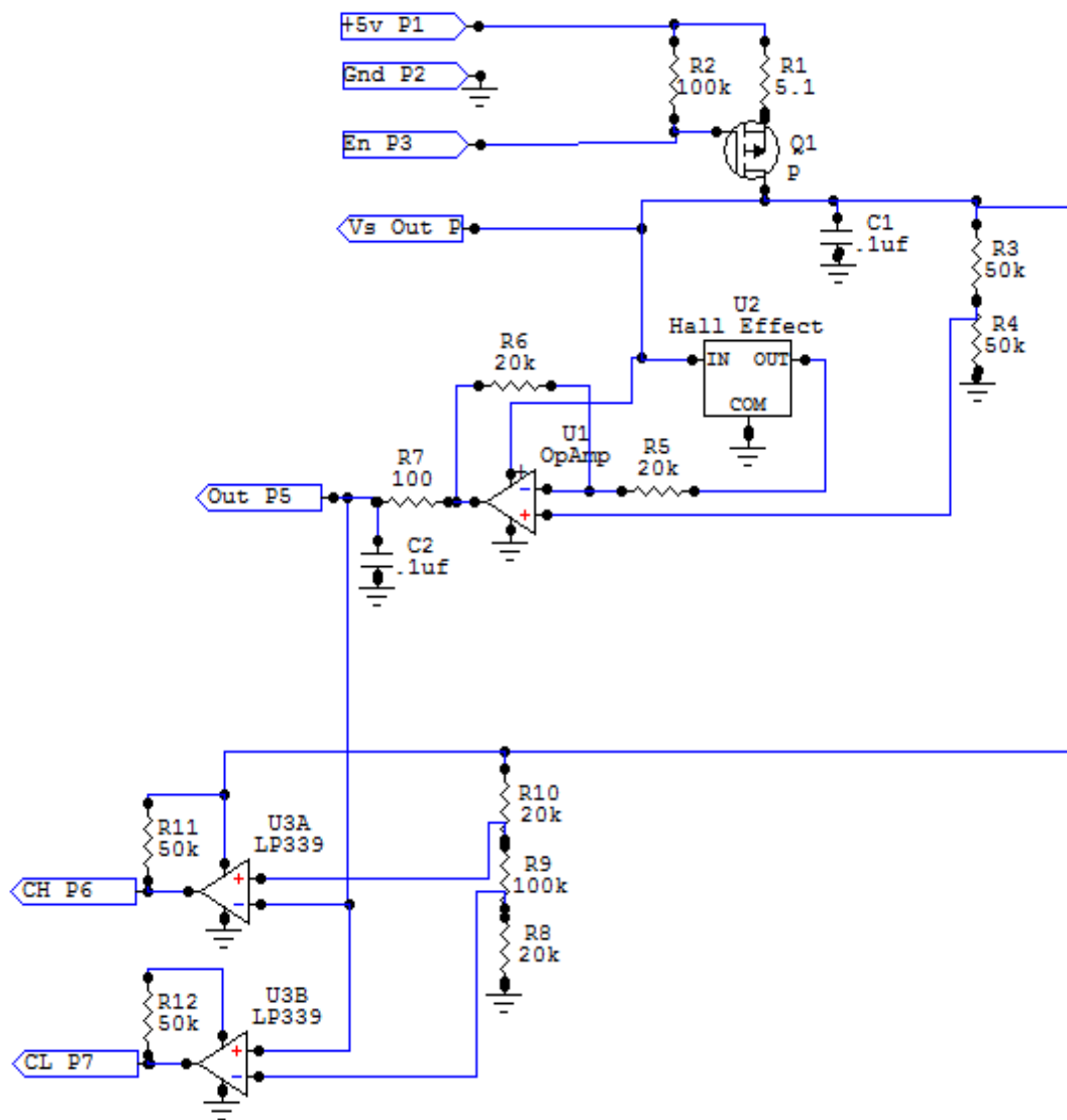
Illustration 1: Current Schematic (subject to change)
